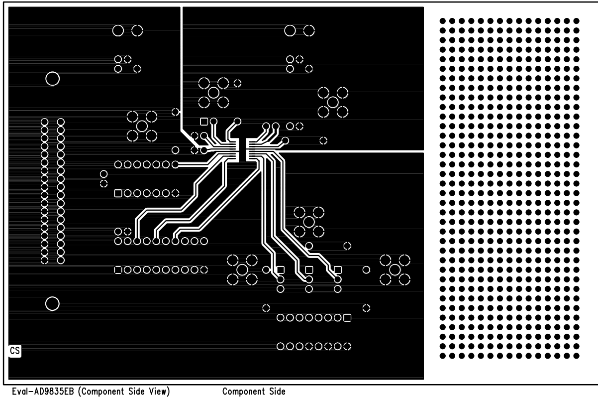
Figure 6. Eval-AD9835EB Component Side Artwork
