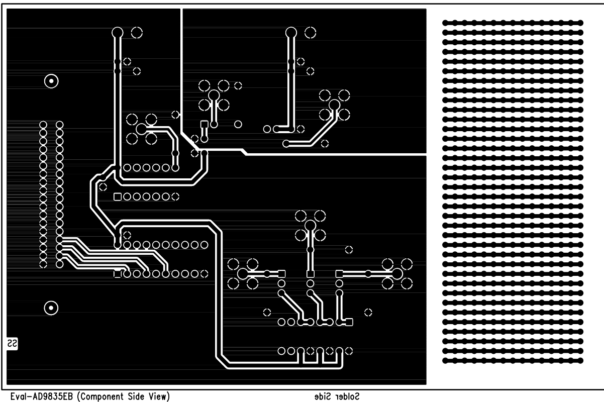
Figure 7. Eval-AD9835EB Solder Side Artwork
