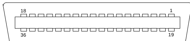
Figure 2: Pin Configuration for 36-Way Connector, J1.
