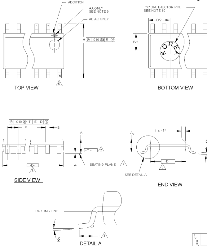
8-Pin Small Outline Integrated Circuit (SOIC, 150-mil)
