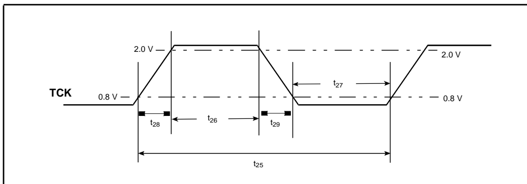
Figure 10. TCK Waveform
