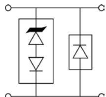
FIGURE 3 Optional Unidirectional configuration (TVS and separate rectifier diode in parallel)
