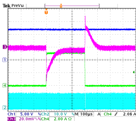
Figure 8 • Transient Response 0A to 5A (5A/μs) CH1 VIN, CH2 Switch Node Voltage, CH3 VOUT (AC coupled across Ceramic Output Capacitors), CH4 Load Current
