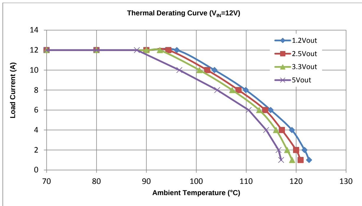
Figure 20 • Thermal Derating Curve (VIN = 12V) Thermal performance shown requires use of thermal vias on all power components and large copper planes.
