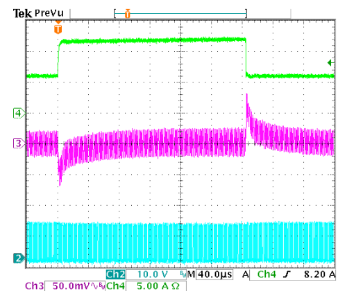
Figure 15 • Transient Response 6A to 12A (5A/µs) CH2 Switch Node Voltage, CH3 VOUT (AC coupled across ceramic output capacitors), CH4 Load Current
