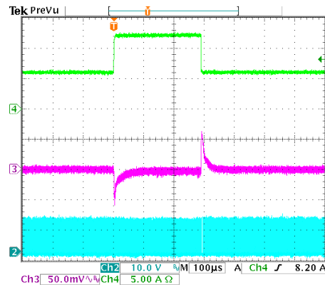
Figure 9 • Transient Response 6A to 12A (5A/μs) CH2 Switch Node Voltage, CH3 VOUT (AC coupled across Ceramic Output Capacitors), CH4 Load Current
