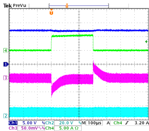
Figure 14 • Transient Response 0A to 5A (5A/µs) CH1 VIN, CH2 Switch Node Voltage, CH3 VOUT (AC coupled across ceramic output capacitors), CH4 Load Current
