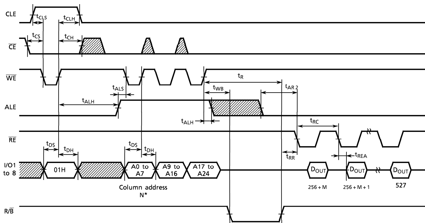
Read Cycle (2) Timing Diagram
