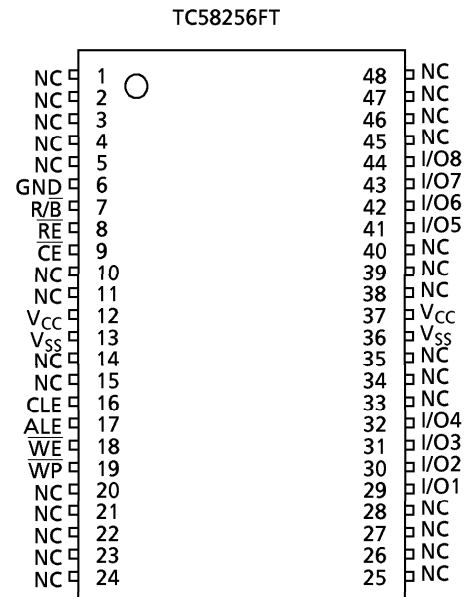
Figure 1. Pinout
