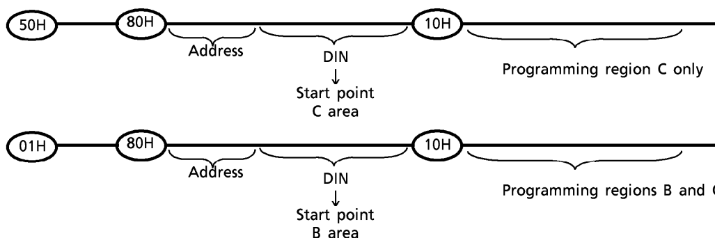
Figure 15. Example of How to Set the Pointer
