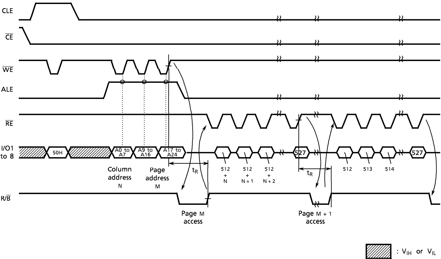
Sequential Read (3) Timing Diagram
