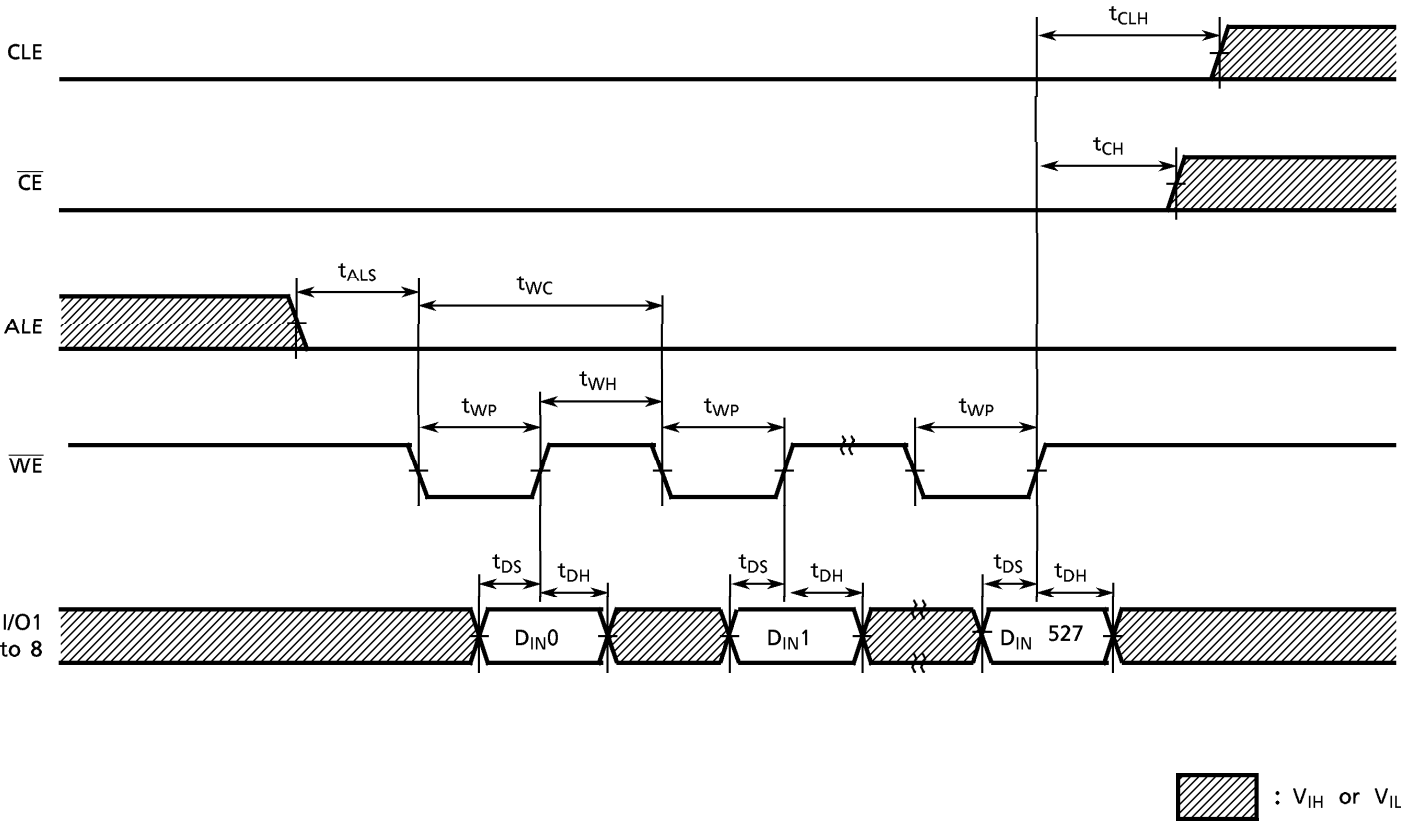
Data Input Cycle Timing Diagram
