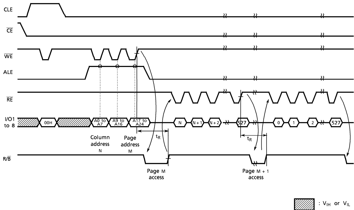
Sequential Read (1) Timing Diagram
