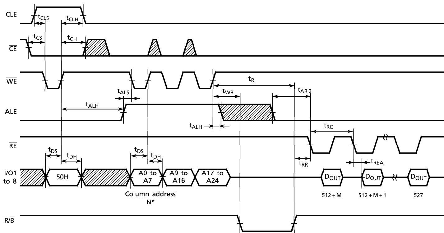
Read Cycle (3) Timing Diagram
