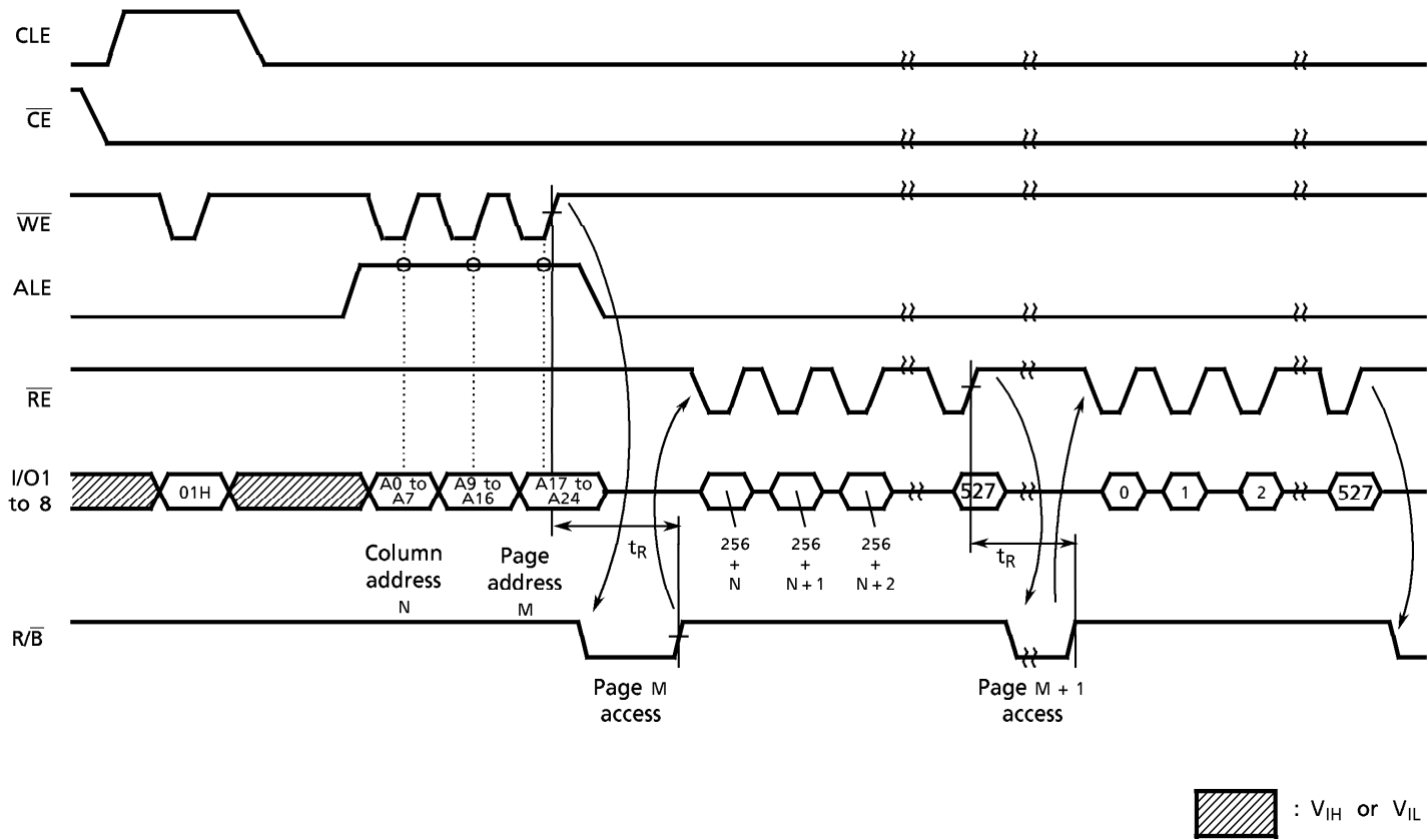
Sequential Read (2) Timing Diagram
