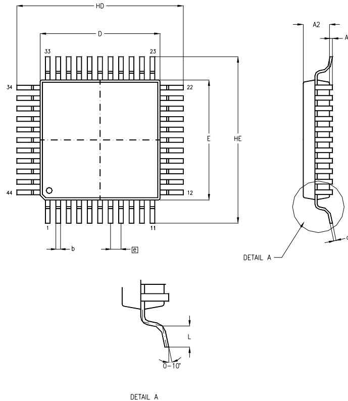
Figure 50. 44-Pin OFP Package Diagram
