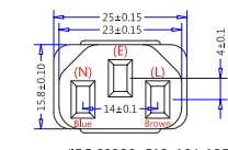
(IEC 60320, C13, 10A 125V~) (Dimensions of Connector Face)
