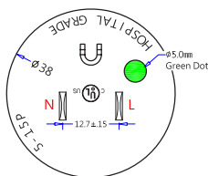
(NEMA 5-15P, Hospital Grade) (Dimensions of Plug Face)
