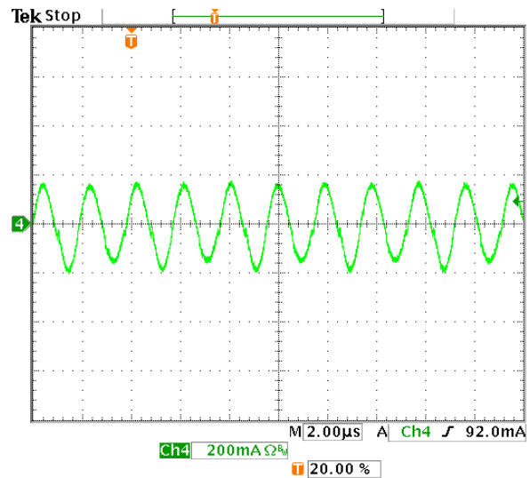
Fig.5.0V-10: Input reflected ripple current, I_c (200mA/div), measured through 10µH at the source at full rated load current and V_{in}=48V . Time scale: 2µs/div.
