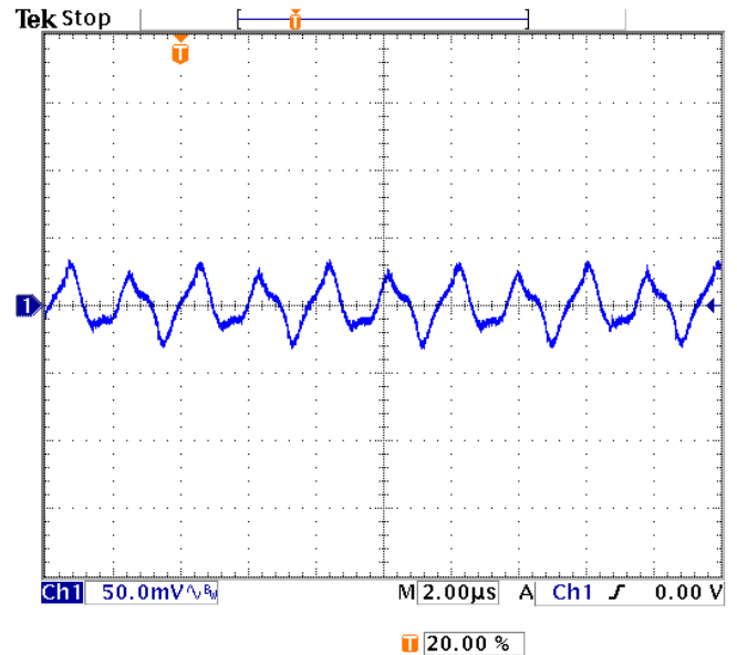
Fig.5.0V-7: Output voltage ripple (50mV/div) at full rated load current into a resistive load with Co=10µF tantalum + 1µF ceramic and Vin=48V. Time scale: 2µs/div
