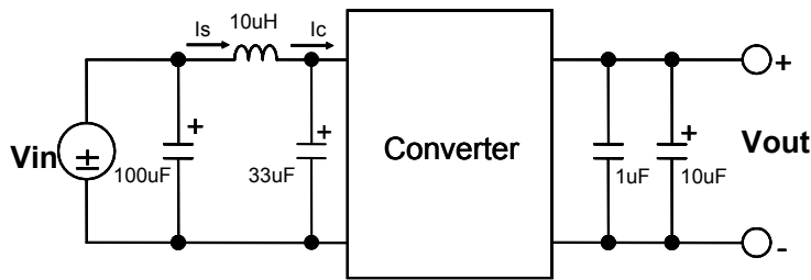
Fig.5.0V-8: Test Set-up for measuring input reflected current.
