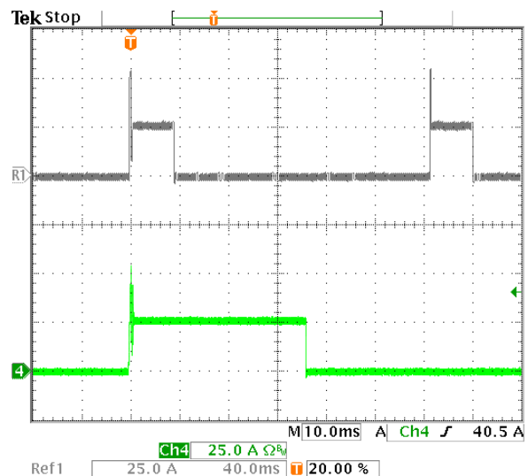
Fig.5.0V-12: Load current (top trace, 25A/div, 40ms/div) into a 10mΩ short circuit during restart, at V_{in} = 48V . Bottom trace (25A/div, 10ms/div) is an expansion of the top trace.
