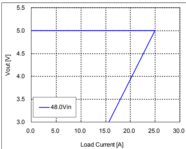
Fig.5.0V-11: Output voltage vs. load current showing current limit point and converter shutdown point. ( V_{in} = 48V )
