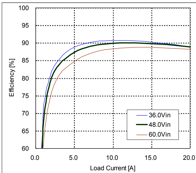
Fig.5.0V-2: Efficiency vs. load current and input voltage for converter mounted horizontally with airflow from pin 3 to pin 1 at a rate of 300LFM (1.5m/s) and Ta=25°C.
