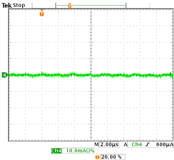
Fig.5.0V-9: Input reflected ripple current, I_s (10mA/div), measured through 10µH at the source at full rated load current and V_{in}=48V . Time scale: 2µs/div.
