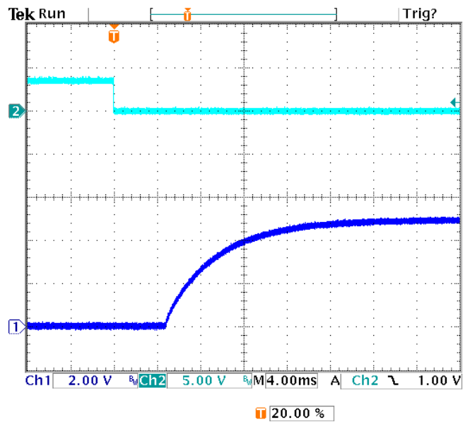
Fig.5.0V-5: Turn-on transient at full rated load current (resistive) plus 10,000µF at Vin=48V, triggered via ON/OFF pin. Top trace: ON/OFF signal (5V/div). Bottom trace: output voltage (2V/div). Time scale: 4ms/div
