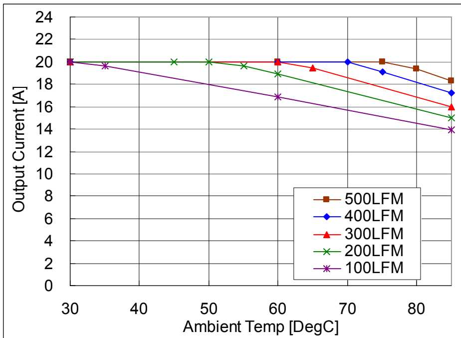
Fig.5.0V-1: Available load current vs. ambient temperature and airflow rates for Vin=48V. Maximum component temperature \leq 125^{\circ}\text{C}
