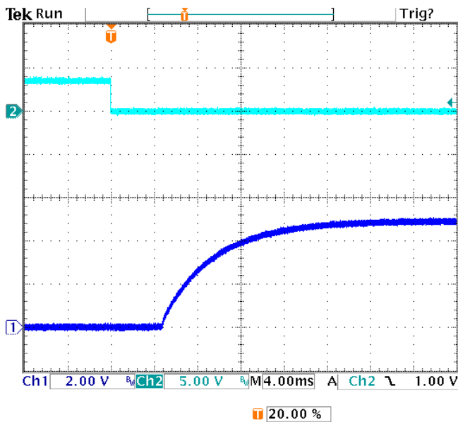
Fig.5.0V-4: Turn-on transient at full rated load current (resistive) with 10µF tantalum + 1µF ceramic capacitor at Vin=48V, triggered via ON/OFF pin. Top trace: ON/OFF signal (5V/div). Bottom trace: output voltage (2V/div). Time scale: 4ms/div
