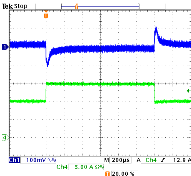
Fig.5.0V-6: Output voltage response to load current step-change (10A↔15A) at Vin=48V. Top trace: Output voltage (100mV/div). Bottom trace: load current (5A/div). Current slew rate: 5A/µs. Co=470µF os-con + 10µF tantalum + 1µF ceramic. Time scale: 200µs/div
