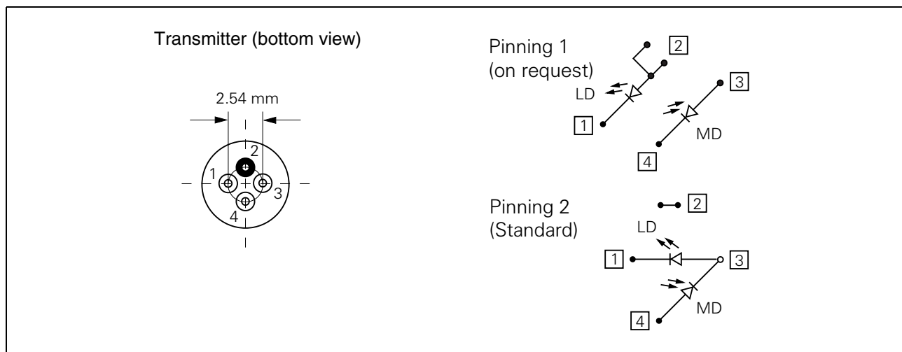
Figure 1 Transmitter
