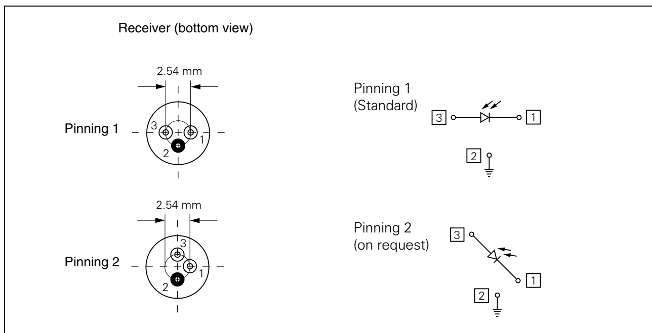
Figure 2 Receiver
