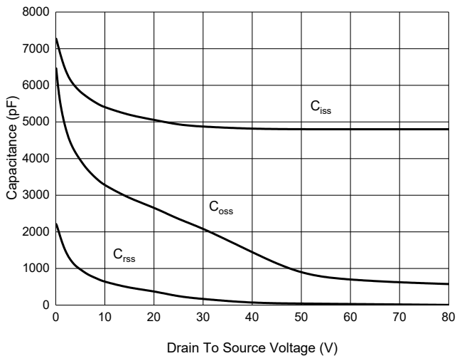
Fig. 5 - Capacitance Characteristics
