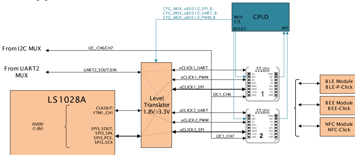
Figure 21. mikroBUS architecture
