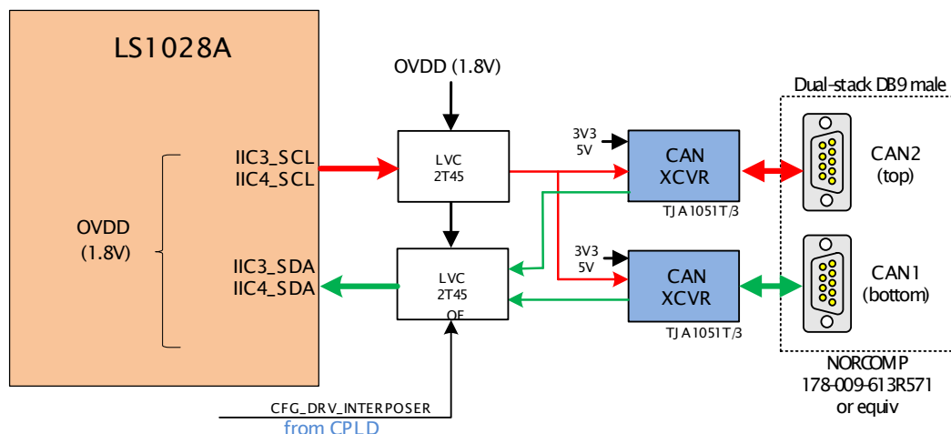
Figure 15. CAN architecture
