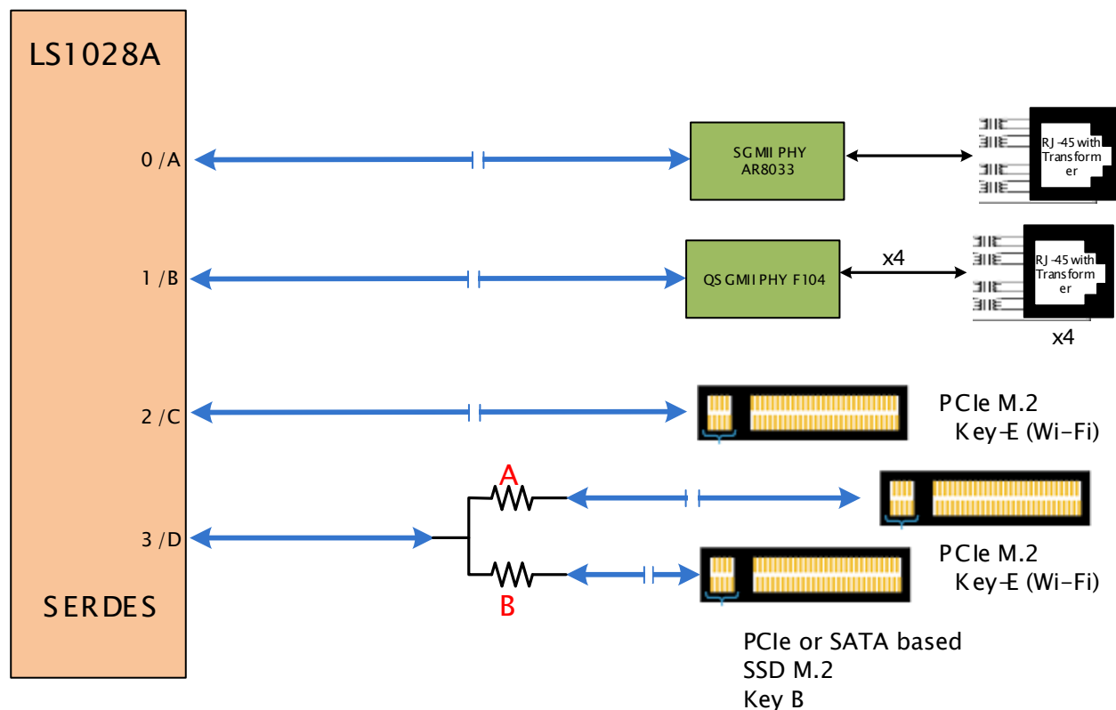
Figure 10. SerDes architecture
