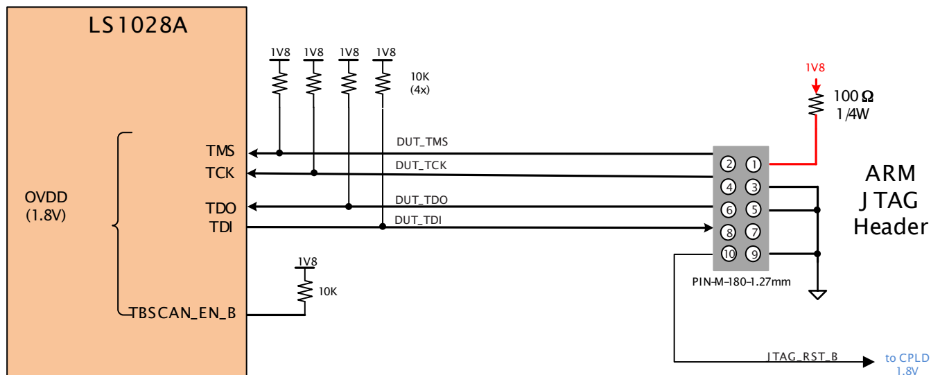
Figure 19. JTAG architecture
