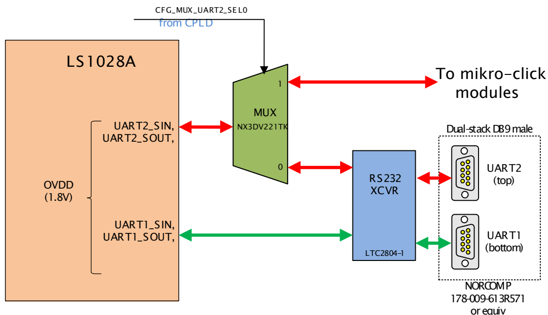
Figure 14. DUART architecture
