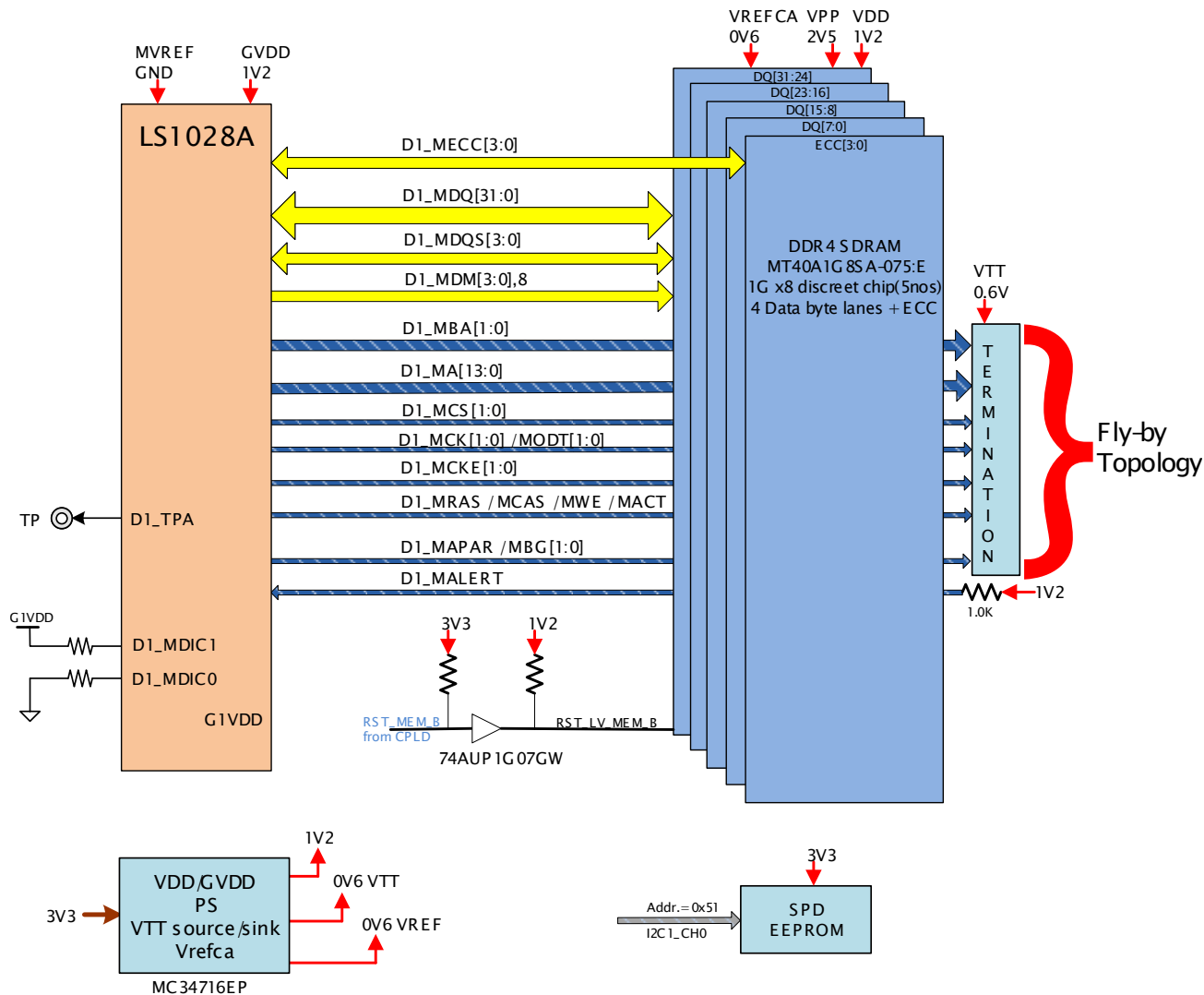
Figure 8. DDR4 interface
