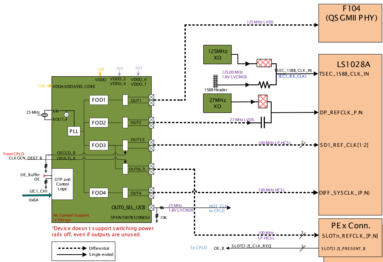
Figure 7. LS1028ARDB clock architecture
