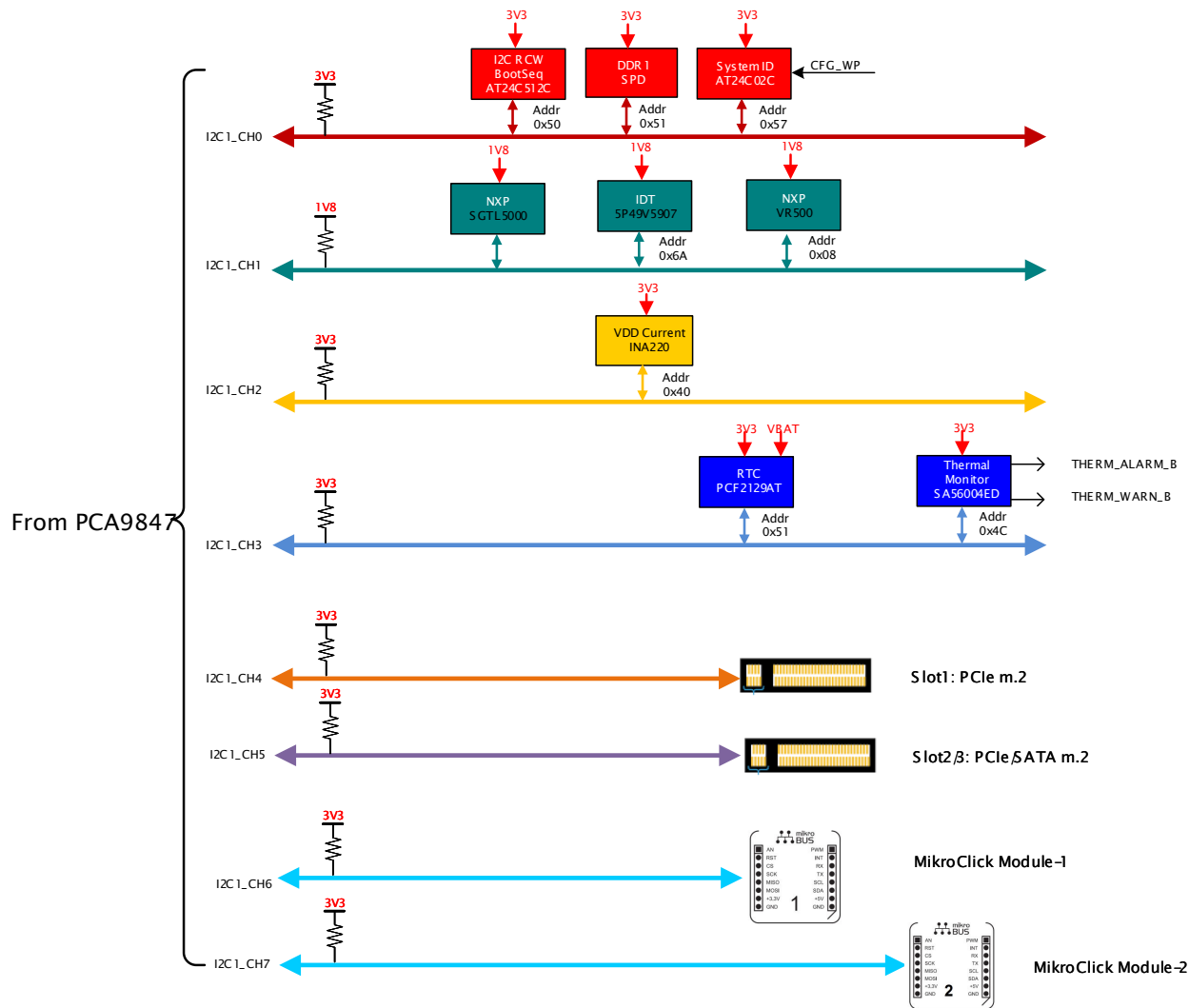
Figure 17. I2C1 channels
