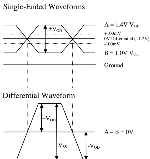
Figure 4: Single-ended & Differential Waveforms
