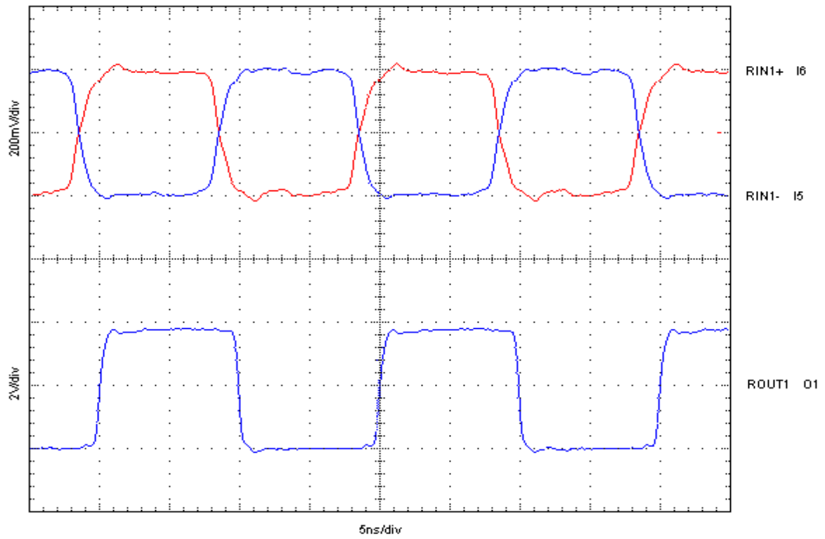
Figure 10: LVDS Cannel #1B Waveforms – A Small Amount of Common Mode Noise Coupled from Output to Input
