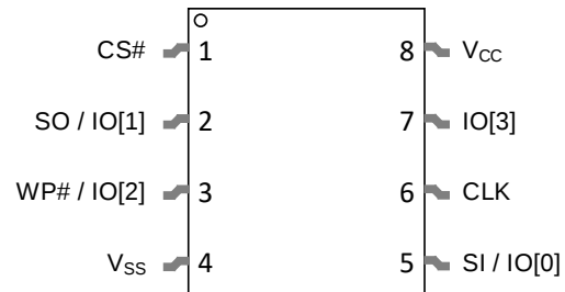
Figure 4: 8-Pin SOIC
