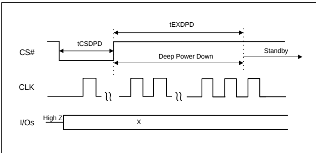
Figure 41: Exit Deep Power Down by Toggling CS#
