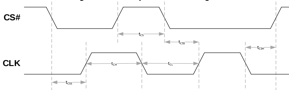
Figure 30: CS# Operation & Timing
