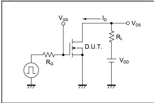
Fig. 1-1 SWITCHING TIME MEASUREMENT CIRCUIT
