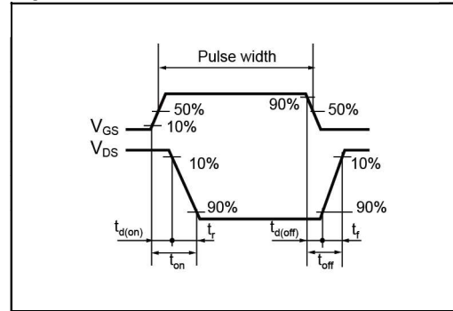
Fig. 1-2 SWITCHING WAVEFORMS
