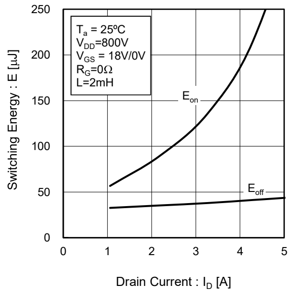
Fig.20 Typical Switching Loss vs. Drain Current
