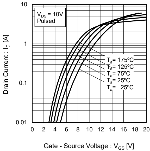
Fig.8 Typical Transfer Characteristics (I)
