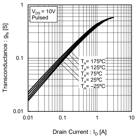
Fig.11 Transconductance vs. Drain Current
