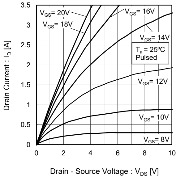
Fig.4 Typical Output Characteristics(I)
