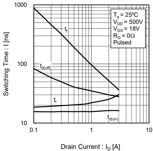
Fig.17 Switching Characteristics
